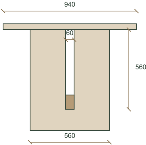
07 / COMPONENT DIMENSIONS
